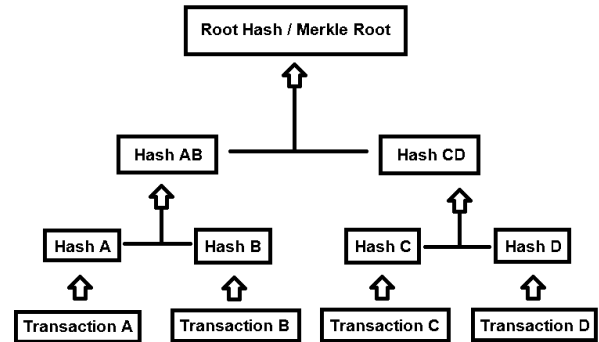
Fig 4: Merkle Root
